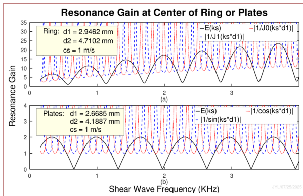
Fig. 3. Resonance gains of shear waves over frequency (no attenuation). (a) Resonance gain of the shear wave produced by a cylindrical ring of radiation force (see Fig. 1(a)). (b) Resonance gain of the shear wave produced by two plates of radiation force (see Fig. 1(b)).
