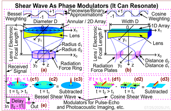
Fig. 1. Generation of shear waves for super-resolution imaging [15] via a phase modulation of the point spread function (PSF) of imaging systems such as pulse-echo and photoacoustic imaging [23]. (a) A cylindrical ring of radiation force produced near the focal distance by a focused Bessel beam (or its piecewise or binary approximation) that is generated with an annular or a 2D array transducer to produce a focused shear wave. (b) The same as (a) except that two plates of radiation force are produced by a focused cosine beam [22] or its binary approximation that is generated by a 1D array transducer. (c1), (c2), and (c3) are propagating shear waves produced by the radiation force in (a) at two different times t_2 and t_1 (either t_2 > t_1 or t_2 < t_1 ), and their subtracted version, respectively, to reduce the sidelobes in the modulated imaging waves. (d1), (d2), and (d3) are the same as (c1), (c2), and (c3) respectively except that the cosine shear waves are produced by the linear array in (b). (e) A sensitive and high-dynamic range interferometer method that is applicable to both (a) and (b) to perform a subtraction or phase-difference detection of modulated imaging-waves [15].
